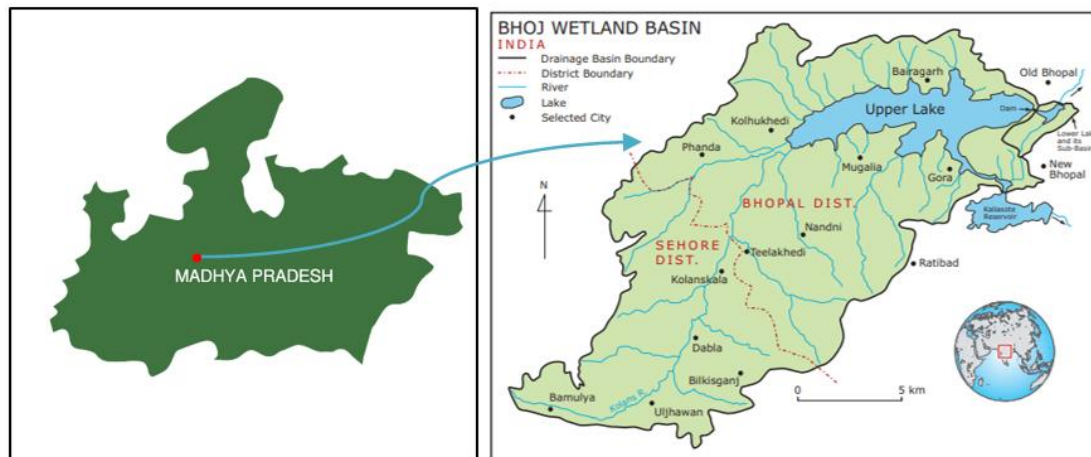
Fig. 1. Map showing Upper Lake Bhopal, Madhya Pradesh (India)
