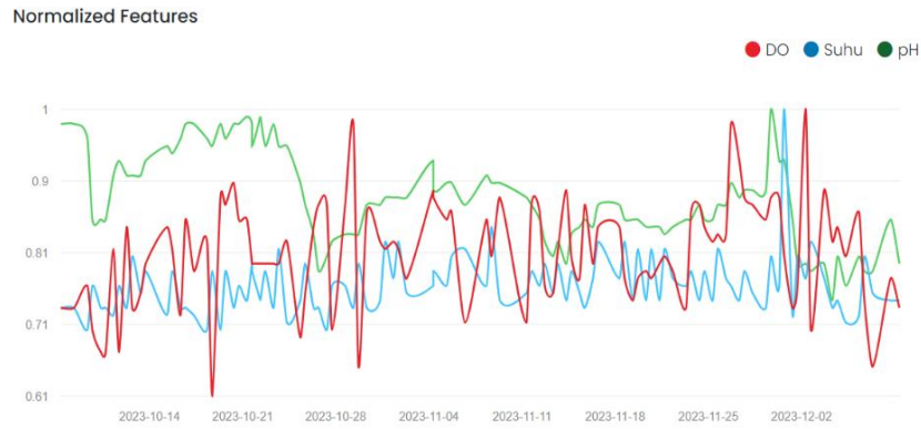
Fig. 8. Combined water quality data chart
