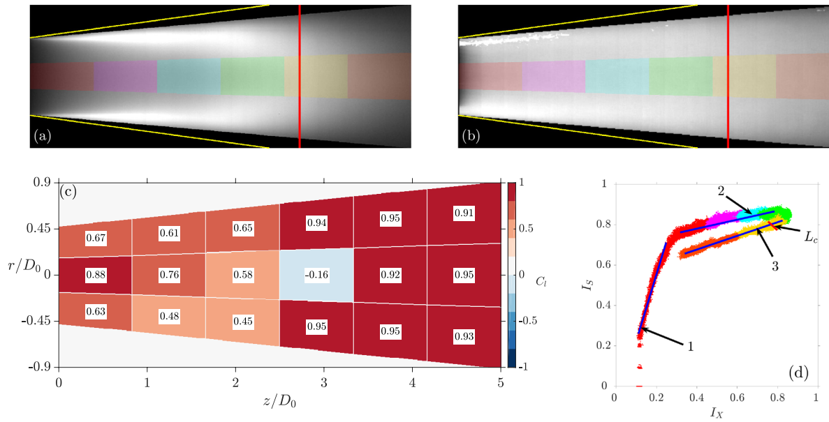
Figure 7. A comparison of the greyscale intensities at identical coordinates along the streamwise direction, from the two measurement techniques. Here, \sigma = 0.60 . (a) Time-averaged x-ray image with the regions of interest superimposed in different colours, (b) time-averaged shadowgraphy image with the regions of interest superimposed in different colours, (c) local correlation coefficients at the different zones, (d) the colour-coded zonal scatter plots. The colours in this scatter plot correspond with the respective coloured regions of interest demarcated in (a) and (b). The vertical red lines in (a) and (b) denote the streamwise location of the estimated cavity length. The red line in (d) is the approximate location of the estimated cavity length along the loop-like trajectory in the scatter plot, while the blue lines in (d), labeled from 1–3, identify the different regimes. In (a) and (b), darker regions represent the liquid phase while the lighter regions represent the vapor phase. The yellow lines in (a) and (b) denote the venturi walls.
