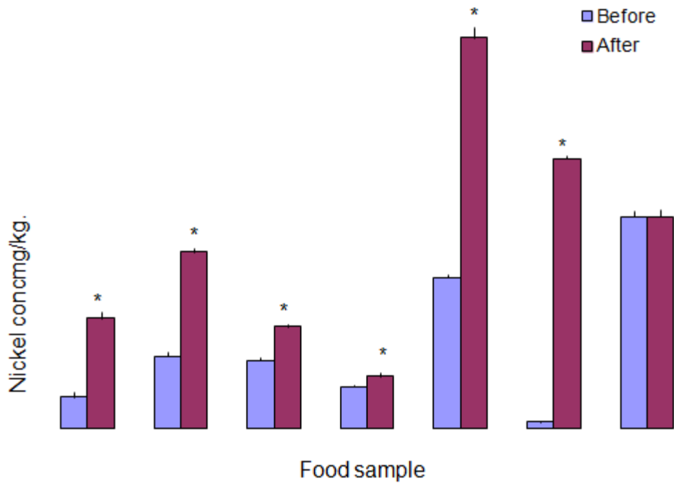
Fig. 3. Comparison of concentration of nickel before and after exposure in the different food samples
