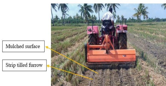
Fig. 5. Mulching cum strip tillage operation by stubble managing unit of the proposed machine
