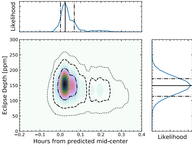
Figure 9. Joint posterior distributions of eclipse depth and time of eclipse center from the analysis plotted in Figure 2. The eclipse depth exhibits no covariance with the eclipse timing, despite the latter’s long tail toward high values.
