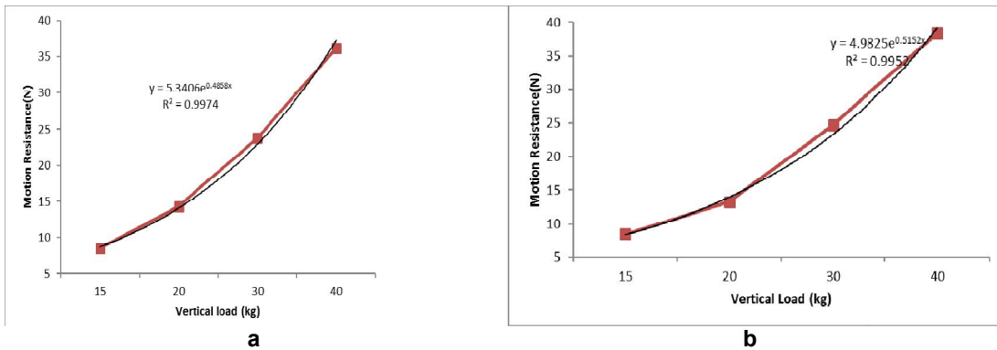
Fig. 7. (a) Effect of vertical load and inflation pressure (274 kPa) on motion resistance test wheel 1 8% moisture content; (b) Effect of vertical load and inflation pressure (380 kPa) on motion resistance for test wheel 1 at 10% moisture content
