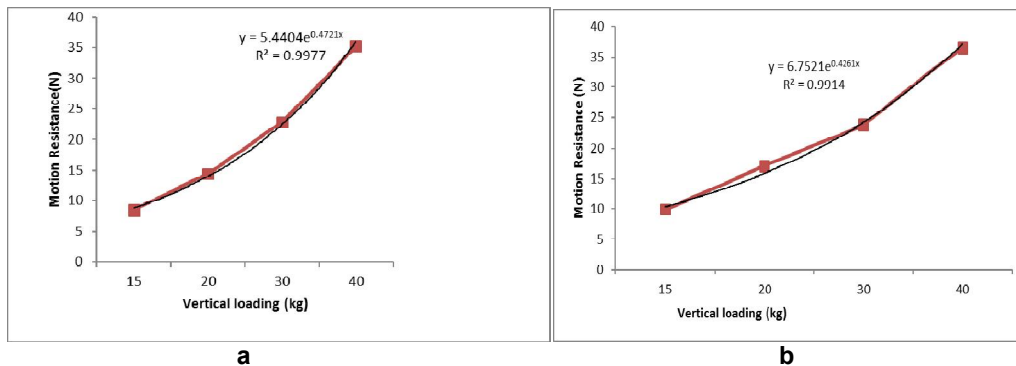
Fig. 8. (a) Effect of vertical load and inflation pressure (274 kPa) on motion resistance test wheel 2 at 8% moisture content; (b) Effect of vertical load and inflation pressure (380 kPa) on motion resistance test wheel 2 at 10% moisture content
