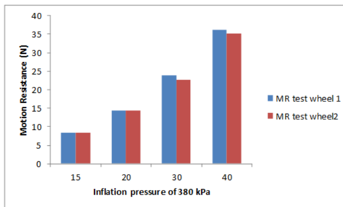
Fig. 12. Motion resistance of pneumatic wheels at 380 kPa inflation pressure and at different weight on clay soil surface at 10% moisture content
