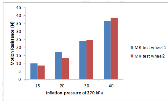
Fig. 11. Motion resistance of pneumatic wheels at 270 kPa inflation pressure and at different weight on clay soil surface at 8% moisture content
