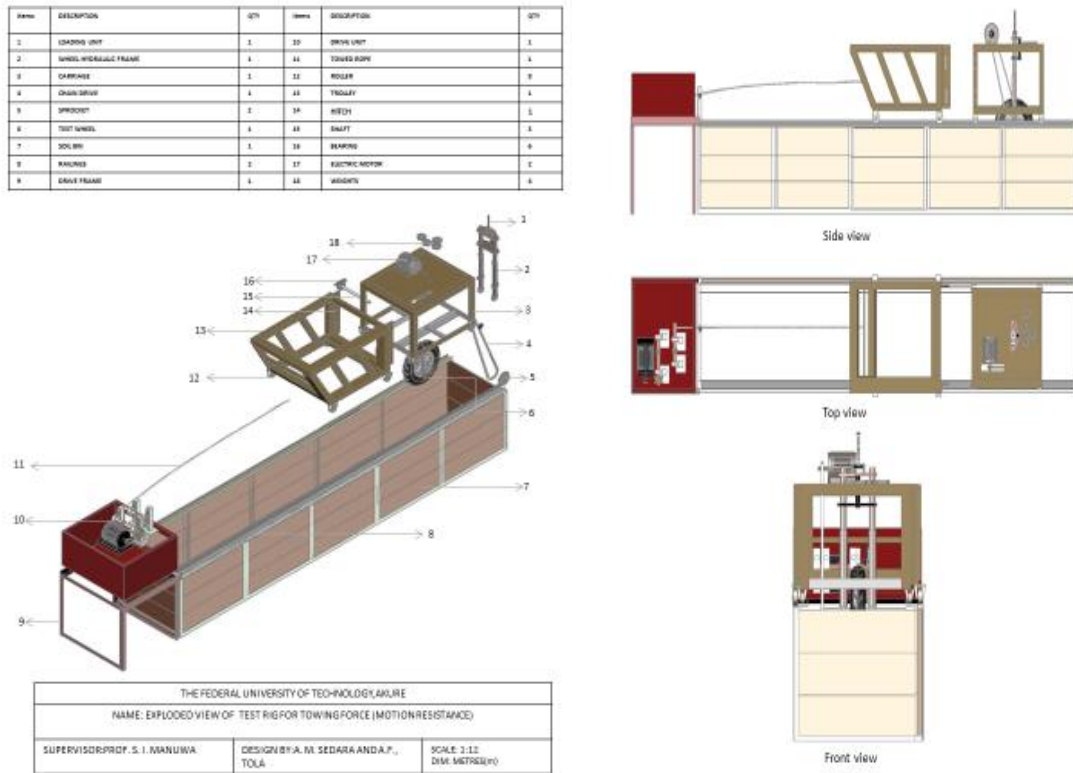
Fig. 2. Exploded and orthographic view of test rig for motion studies (CAD Design)
