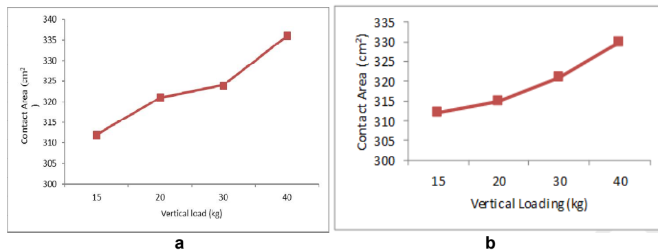
Fig. 9. (a) Effect of vertical load and inflation pressure (270 kPa) on contact area, test wheel 1; (b) Effect of vertical load and inflation pressure (380 kPa) on contact area, test wheel 1
