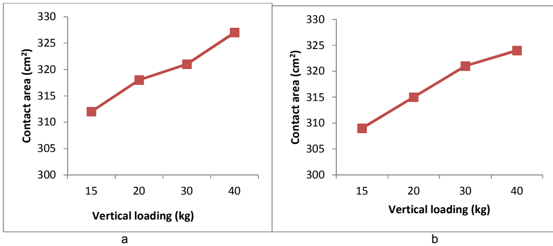
Fig. 10. Effect of vertical load and inflation pressure (270 kPa) on contact area, test wheel 2; (b) Effect of vertical load and inflation pressure (380 kPa) on contact area, test wheel 2
