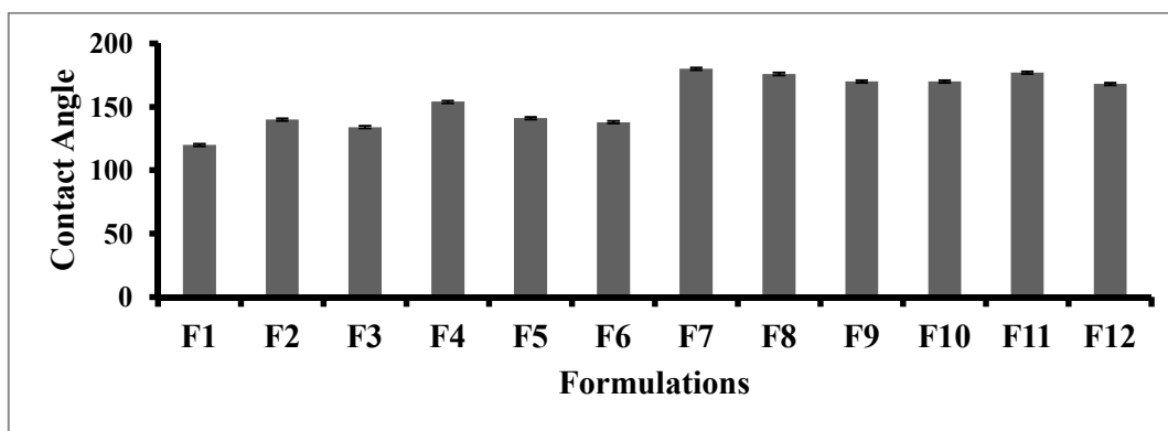
Fig. 12. Graph showing % assay of different formulations from F 1 - F 12 . X-axis represents the formulations and y-axis represents the assay results in percentage. Assay was performed using high-pressure liquid chromatograph that was equipped with a UV detector at 231 nm and connected with computing system. Chromatographic column 25 cm x 4.6 mm (i.d.), 5 \mu Hypersil BDSC18.Glass fiber Filter (type GF/A available from Whatman, 20 \mu\text{L} injection was inserted at a flow rate of 1.5 ml/min at ambient temperature
