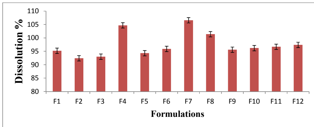
Fig. 14. Graph showing Dissolution of different formulations from F 1 - F 12 in percentage values. X-axis represents the formulations and y-axis represents the dissolution results in percentage. Dissolution studies were performed using high-pressure liquid chromatograph that was equipped with a UV detector at 231 nm and connected with computing system Chromatographic column 25 cm x 4.6 mm (i.d.), 5 \mu Hypersil BDSC18. Glass fiber Filter (type GF/A available from Whatman. 20 \mu\text{L} injection was inserted at a flow rate of 1.5 ml/min at ambient temperature
