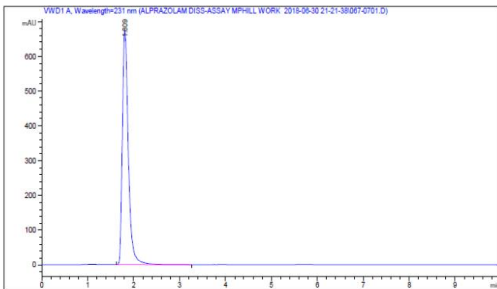
Fig. 15. HPLC Chromatogram of Sample 05A (Assay). X-axis represents the time in minutes and y-axis represents the height of peak in mAU. The graph shows peak area of 6106.45020 mAU at retention time of 1.809 minutes. The height of peak is 674.00757 mAU. High-pressure liquid chromatography was equipped with a UV detector at 231 nm and connected with computing system. Chromatographic column 25 cm x 4.6 mm (i.d.), 5 \mu Hypersil BDSC18.Glass fiber Filter (type GF/A available from Whatman. 20 \mu L injection was inserted at a flow rate of 1.5 ml/min at ambient temperature
