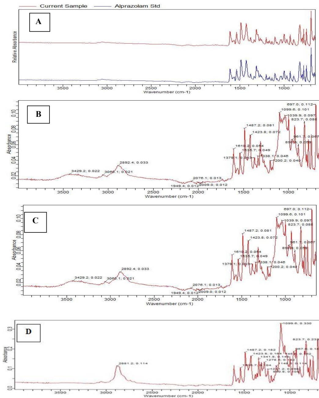
Fig. 3. FTIR spectra of alprazolam standard v/s sample (A), mixture of alprazolam and HPMC E5 (B), mixture of alprazolam and HPMC E15 (C), mixture of alprazolam and PEG 400 (D), mixture of alprazolam and menthol (E), mixture of drug and all the used excipients (F)
