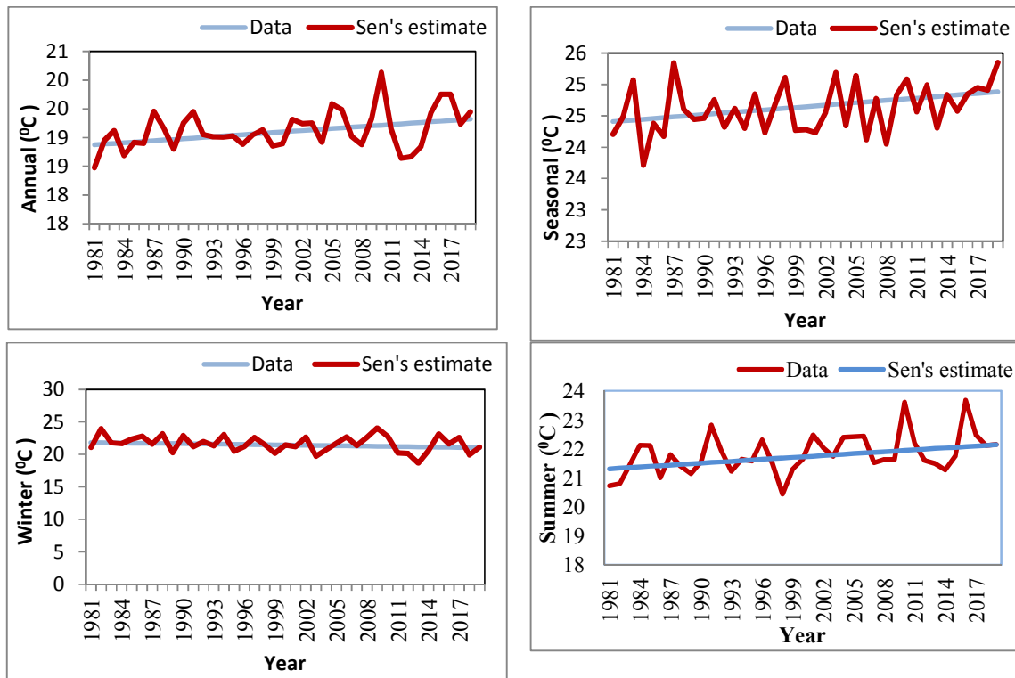
Fig. 5. Minimum temperature variability during the period 1981-2019 for different months, season and annual rainfall
