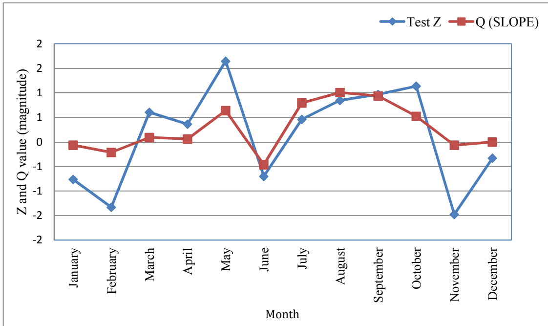
Fig. 2. Plot showing MK statistics (Z value) and Sen's slope (Q value) for rainfall trend analysis
