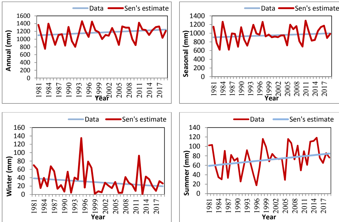
Fig. 3. Variability in rainfall pattern in different months, seasons and annual rainfall Trend analysis of Temperature
