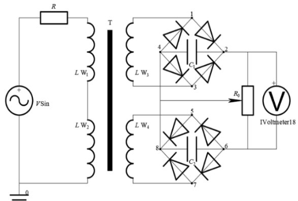
Fig. 6. External circuit
