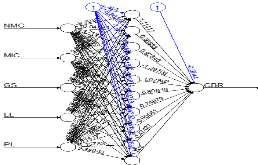
Fig. 1. Neural network plot of CBR
