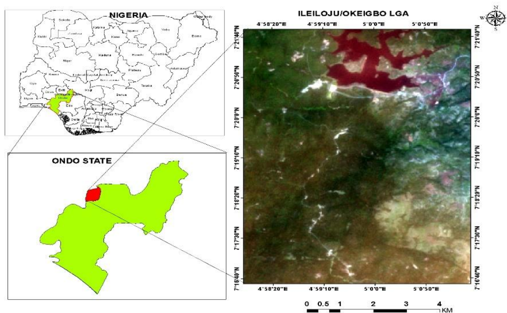
Fig. 1. Map of the study area (Source: Political Map of Nigeria: https://www.worldometers.info )
