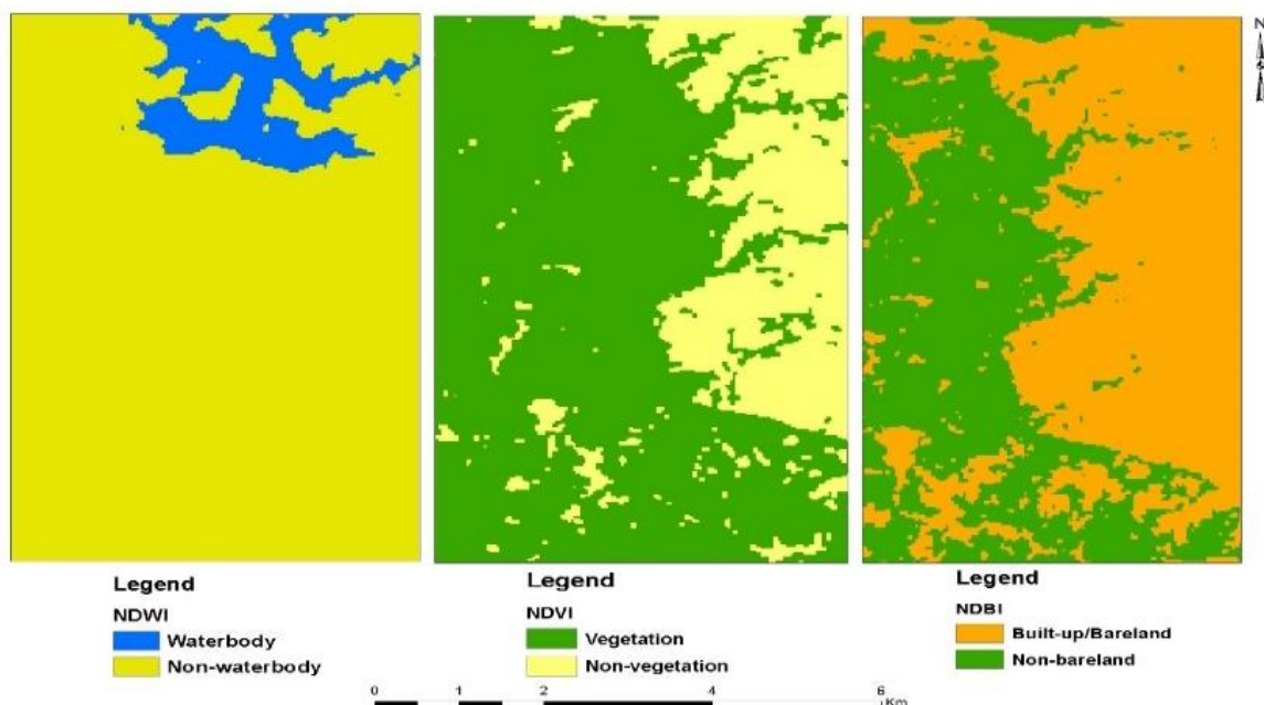
Fig. 4. The index-derived maps of NDVI, NDWI and NDBI
