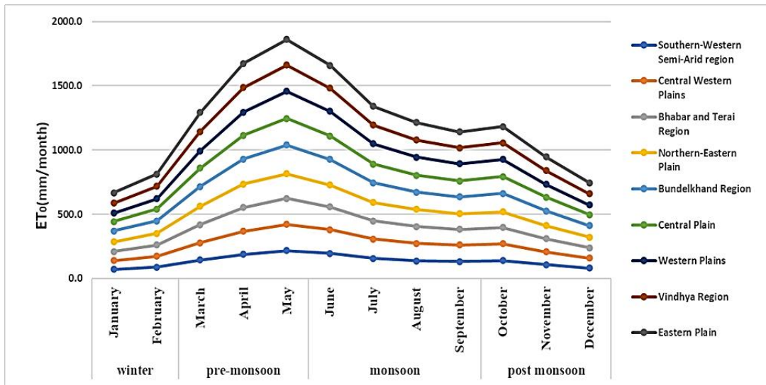
Fig. 1. Reference evapotranspiration
