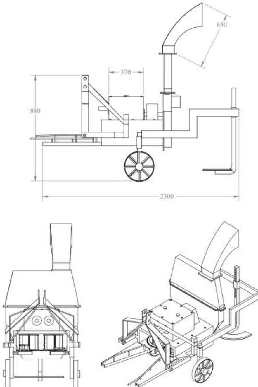
Fig. 1. Schematic diagrams and geometrical model of cotton stalk shredder cum uprooter (all dimension in mm)
