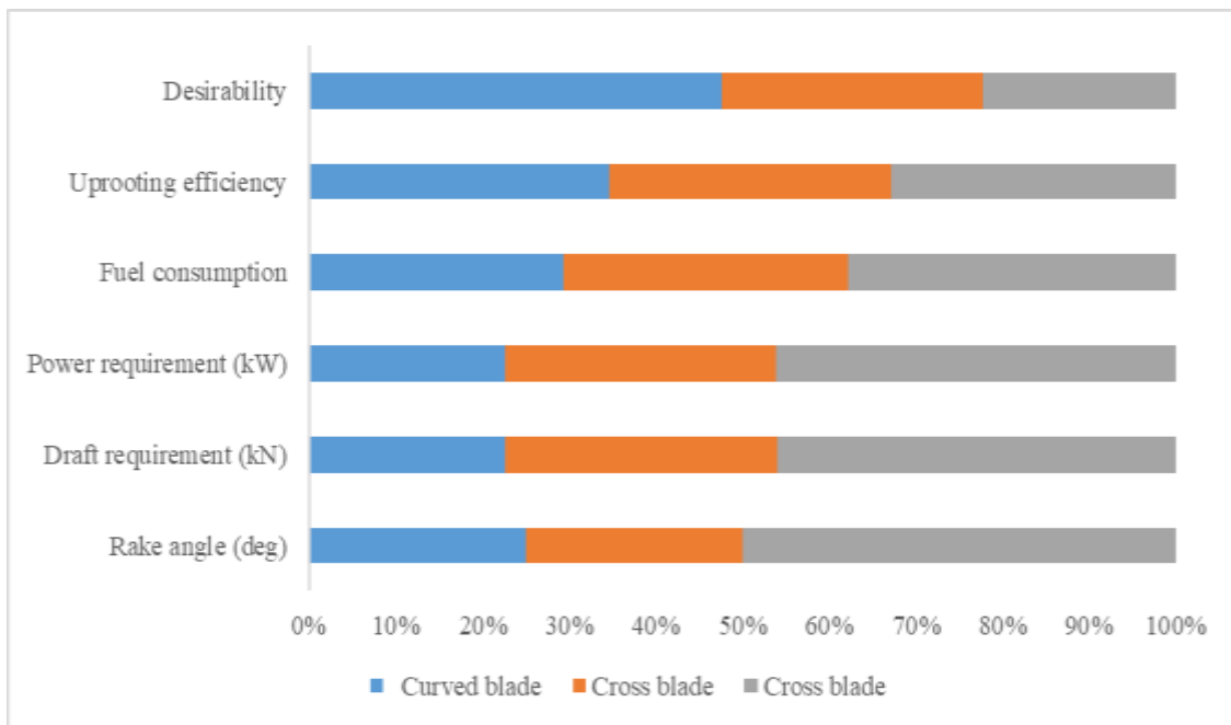
Fig. 6. Desirability graph of cotton stalk shredder cum uprooter
