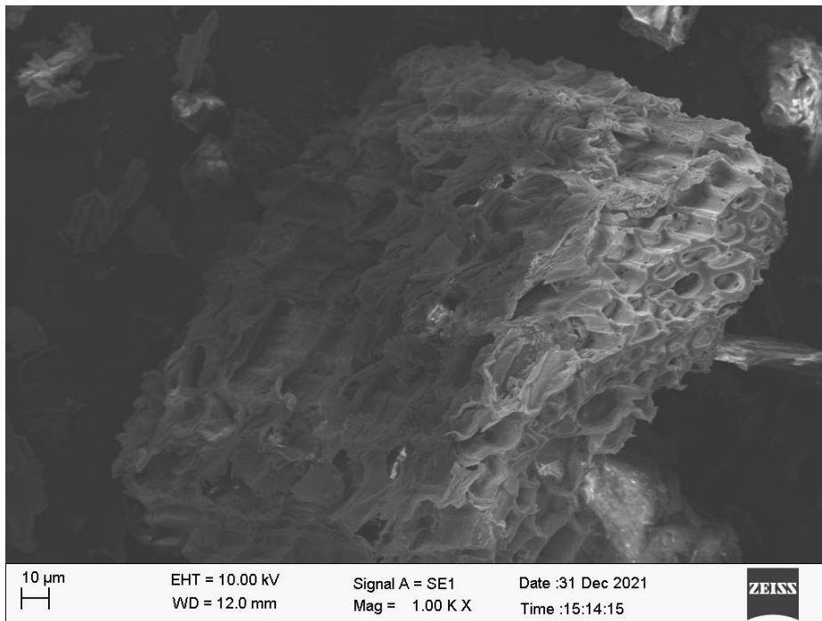
Plate 1. SEM micrographs of paddy husk biochar
