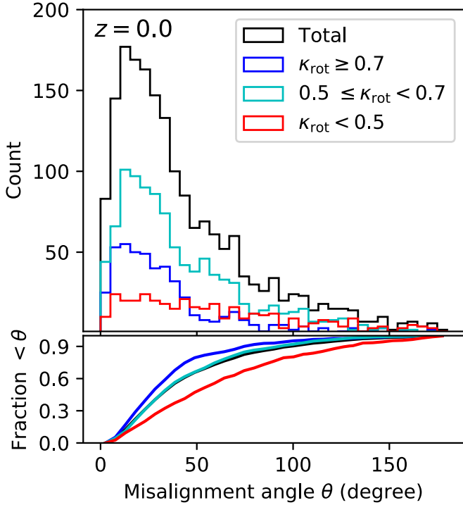
Figure 4. The number distribution of the misalignment angle \theta (top) and its accumulative fraction (bottom) at z=0 . The misalignment angle \theta measures the angle between vectors j_s and j_h . The three groups of galaxies are shown in blue, cyan, and red. The black curve corresponds to the distribution of all central galaxies.
