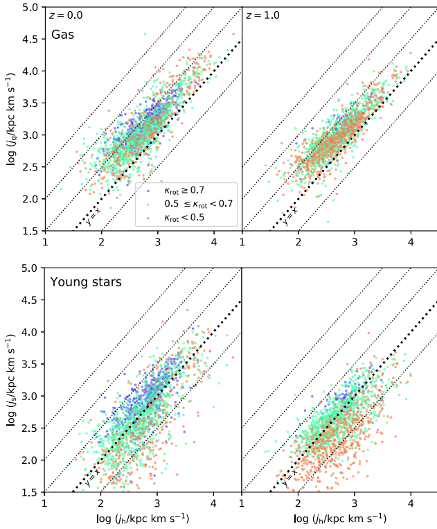
Figure 3. The evolution of the j_s - j_h relation for gas (top) and young stars (bottom) in TNG50 at z = 0 (left) and z = 1.0 (right). The red, green, and blue symbols are central galaxies that correspond to spheroid-dominated galaxies with \kappa_{\text{rot}} < 0.5 , disk-dominated galaxies with 0.5 \leq \kappa_{\text{rot}} < 0.7 , and disk-dominated galaxies with \kappa_{\text{rot}} \geq 0.7 , respectively. The dotted lines highlight the scaling relation in intervals of 0.5 dex. We exclude the cases with star formation rates lower than 0.1 M_{\odot} \text{ yr}^{-1} in the last 1 Gyr (i.e., quenched galaxies), which only contribute a small fraction ( \sim 1/4 at z = 0 ) of even the spheroid-dominated galaxies.
