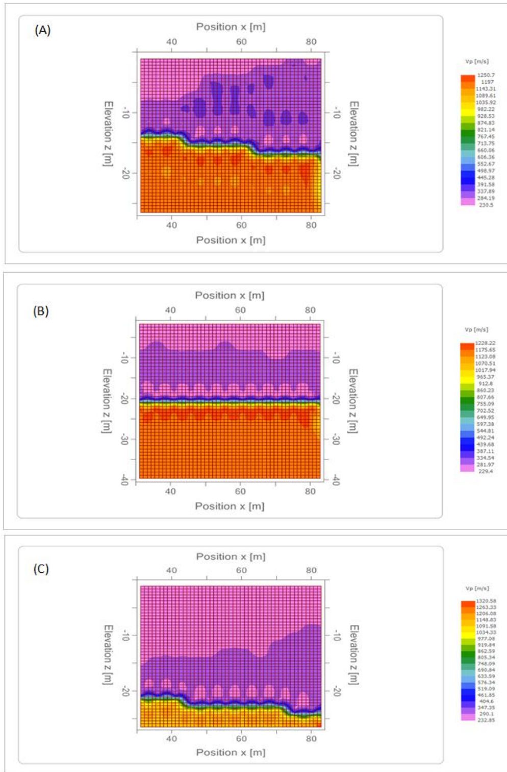
Fig. 3. GRM-depth velocity model for profile 1 to 3 respectively
