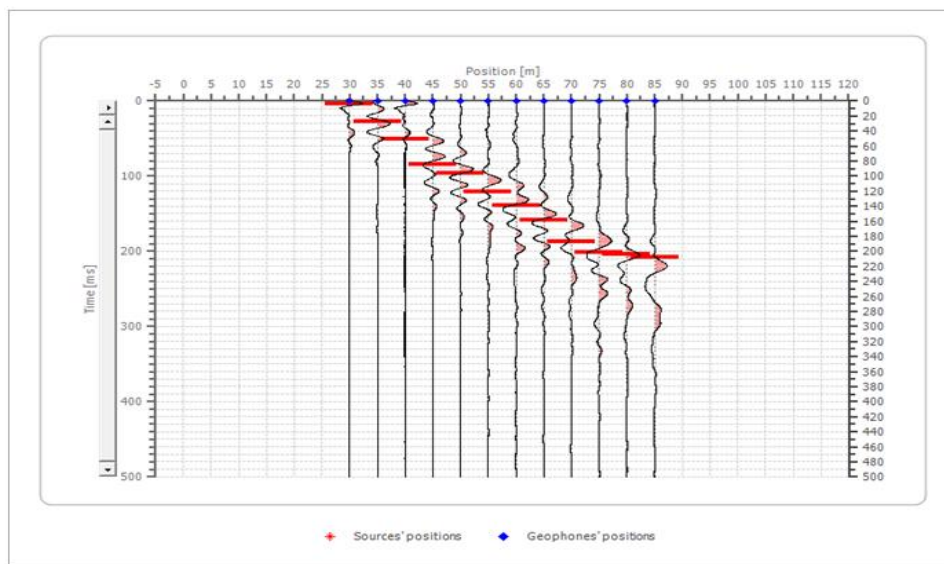
Fig. 2. A sample of a picked first wave arrival time from the collected wave records
