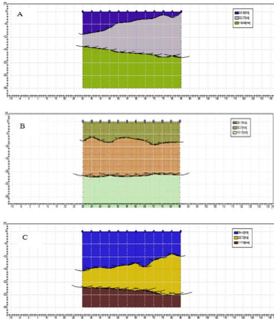
Fig. 4. Morphology of refractor showing seismic velocity of each layer across the three profiles respectively
